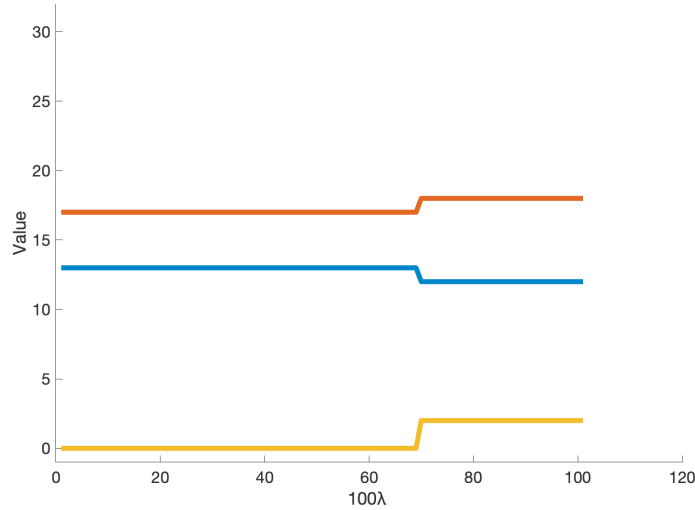
Figure 6: Values of u_L(x_\lambda(\infty)) (blue), of u_R(x_\lambda(\infty)) (orange) and of the number of connected components (yellow) in G_\lambda for \lambda varying between 0 and 1. 100 Simulations were run for values of \lambda between 0 and 1 with a step size of 0.01 (values of \lambda are reported in percentage terms). Values were approximated by setting T = 100 .
