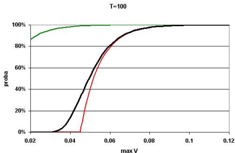
FIGURE 4. Simulated cumulative distribution function (in black) of the maximum step size for the 2-adic attractor, with T = 100 . The simulation has been carried out with 10,000 sets of T variables drawn in the invariant measure of the attractor. In red, we represent the lower bound of the cumulative distribution function (the upper bound of quantiles, equation (23)). In green, we represent the upper bound of the cumulative distribution function (the lower bound of quantiles, equation (24)).
