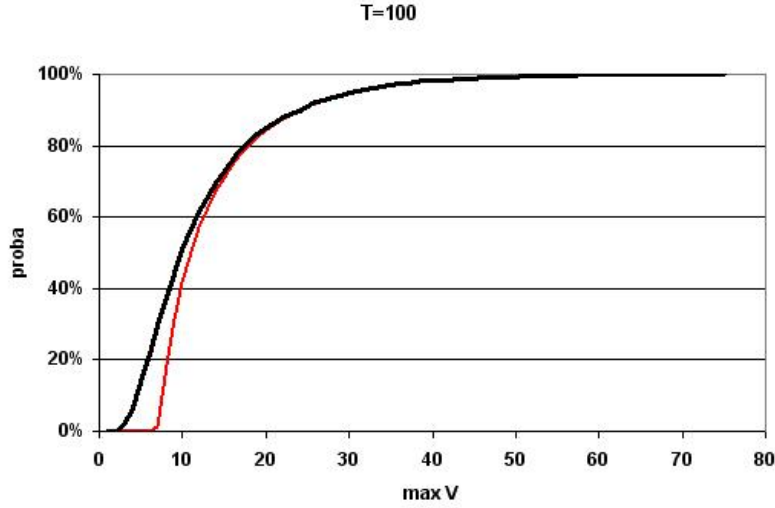
FIGURE 6. Simulated cumulative distribution function (in black) of the maximum step size for exponential random variables, with intensity \lambda = 0.1 and T = 100 . The simulation has been carried out with 10,000 sets of T variables drawn in the exponential probability distribution. In red, we represent the lower bound of the cumulative distribution function (the upper bound of quantiles, equation (26)). Matching the black line, we represent the approximation by the truncated product of the analytic asymptotic cumulative distribution function, equation (27), which coincides with the simulated distribution.
